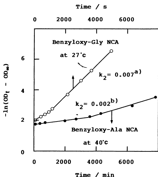
Fig. 1. Pseudo-first-order plots for cyclohexylamine initiated polymerization of N -benzyloxy-NCA of glycine and alanine, as followed by the optical density difference, (OD_t - OD_\infty) , of the anhydride carbonyl group at 1860\text{ cm}^{-1} . [NCA]/[amine]=10 . The corresponding second-order rate constants ( k_2 ) appear along with linear portions of the plots: a) 1\text{ mol}^{-1}\text{ s}^{-1} ; b) 1\text{ mol}^{-1}\text{ min}^{-1} .
